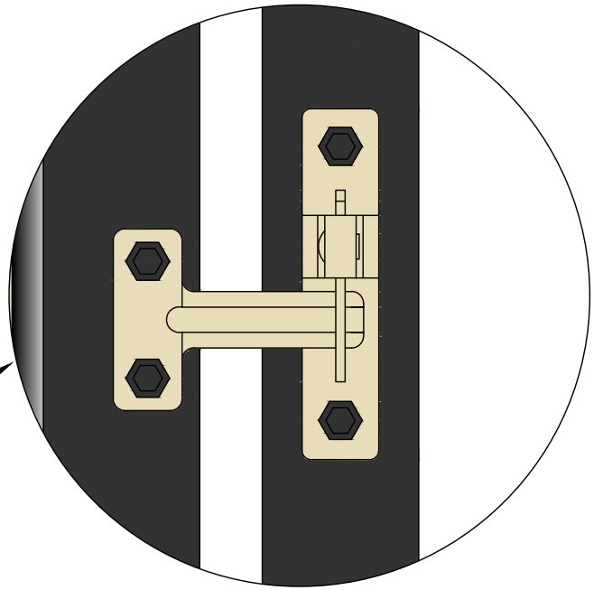
D LATCH & STRIKER Allow 10-15mm for Striker
