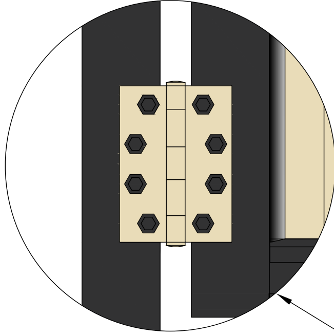
BUTT HINGE Allow 10-15mm for butt hinges
