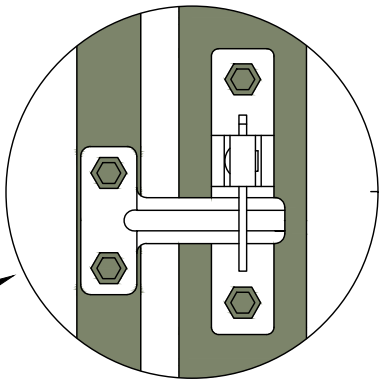
D LATCH & STRIKER Allow 10-15mm for Striker
