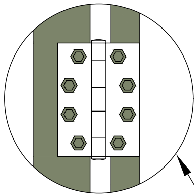
BUTT HINGE Allow 10-15mm for butt hinge
